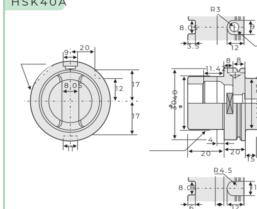
HSK40A
