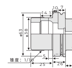
HSK63F
