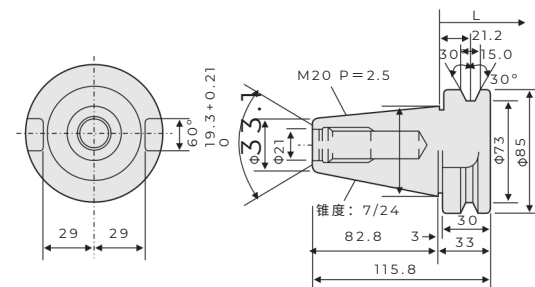
BT45
