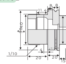
HSK40E
