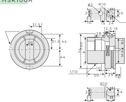
HSK100A
