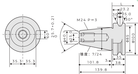
Bt50
