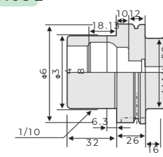
HSK63E
