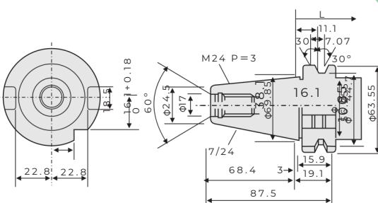
Sk40
