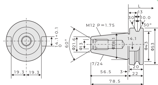
Bt35
